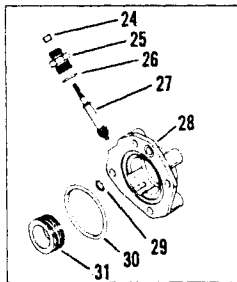
PARKING BRAKE WITH SPEEDO GEAR
