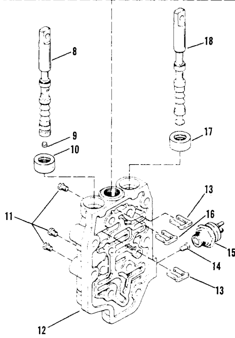
HYDRAULIC DECLUTCH
